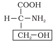
Serine
