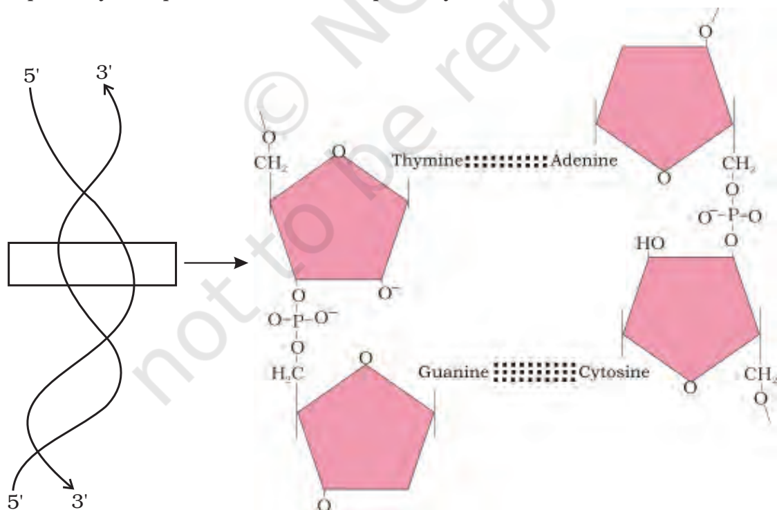
Figure 9.5 Diagram indicating secondary structure of DNA
