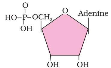
Adenylic acid
