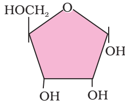
C_5H_{10}O_5 (Ribose)
