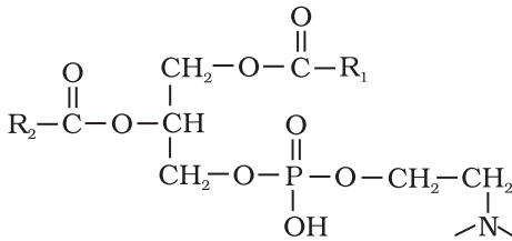
Phospholipid (Lecithin)
