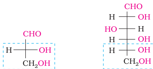
D- (+) - Glyceraldehyde
